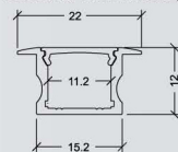
Sectional Dimensions (mm)
